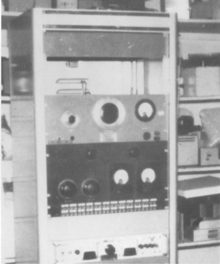
At least one of the first 200A's purchased by Walt Disney for "Fantasia" is still operating efficiently in the Hollywood sound studio, and is seen as the instrument second from the top. The movie itself is seen in revivals from time to time.
